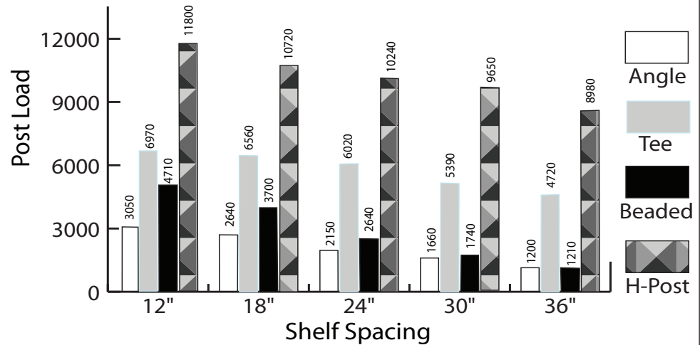
All post capacities shown are based on the latest AISI Design Manual for cold-formed members.
